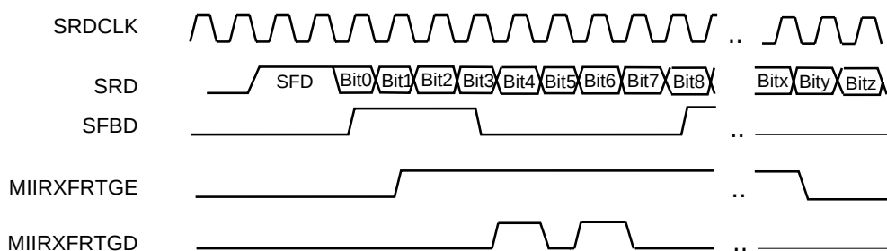
Figure 37. MII Receive Frame Tagging
