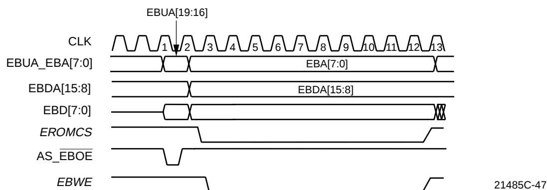
Figure 44. Flash Write from Expansion Bus Data Port
