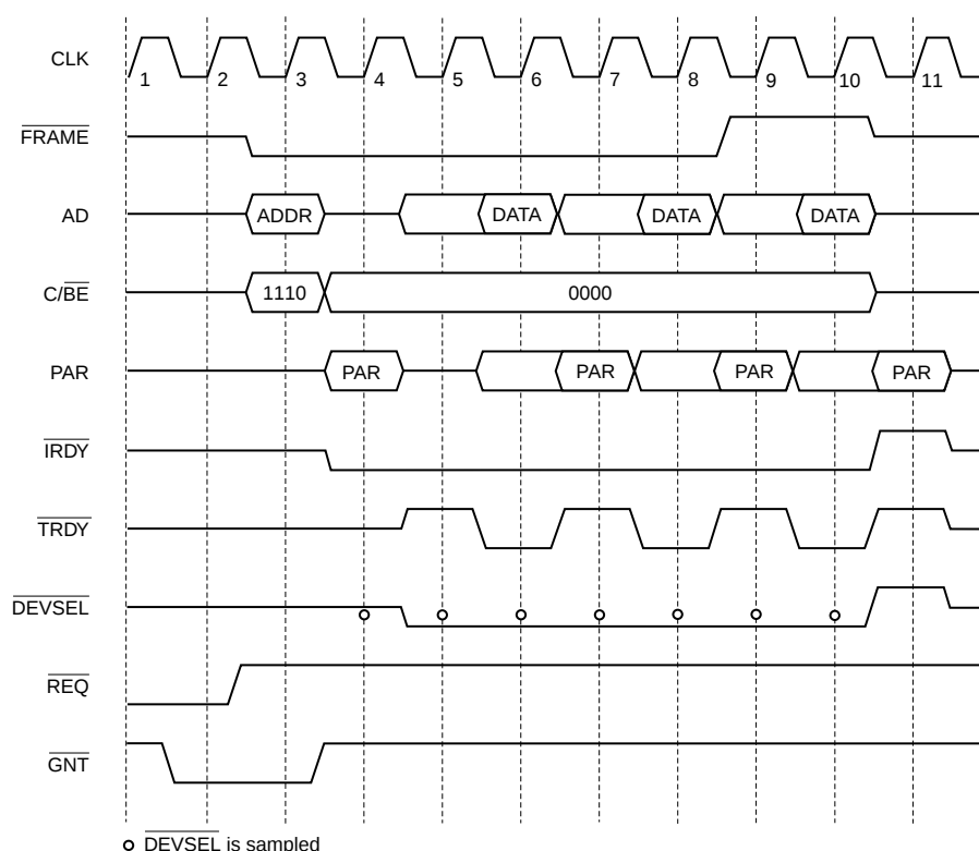
Figure 13. Burst Read Transfer (EXTREQ = 0, MEMCMD = 0)
