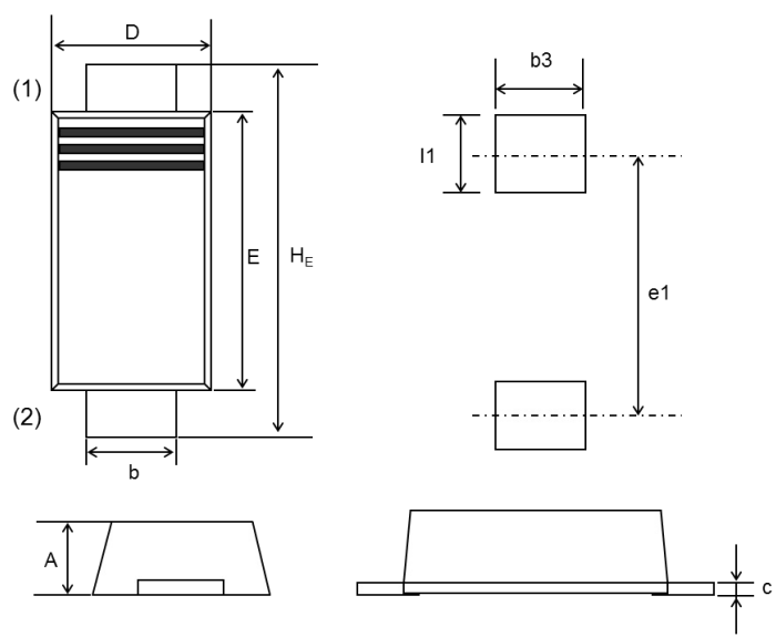
SOD-123FL, (FMDU)
