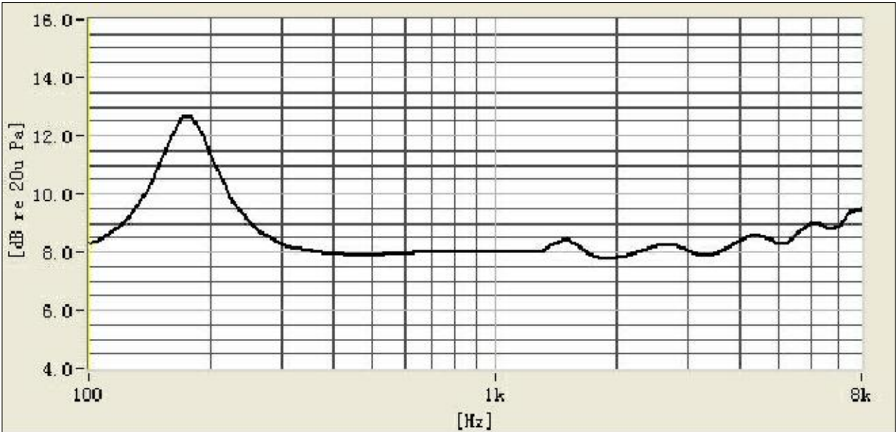
1.6 Rub&Buzz -Active Curve( only for reference)
