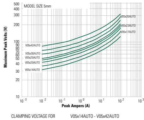
Maximum Clamping Voltage for 5mm Parts V05x14AUTO - V05x42AUTO
