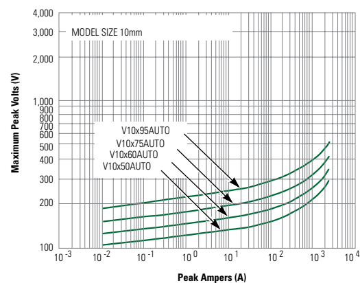
Maximum Clamping Voltage for 10mm Parts V10x50AUTO - V10x95AUTO
