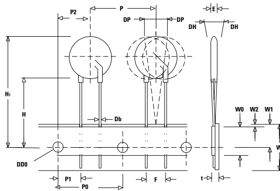
5 and 7mm Devices STRAIGHT LEADS "L1"
