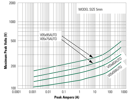
Maximum Clamping Voltage for 5mm Parts V05x50AUTO - V05x95AUTO
