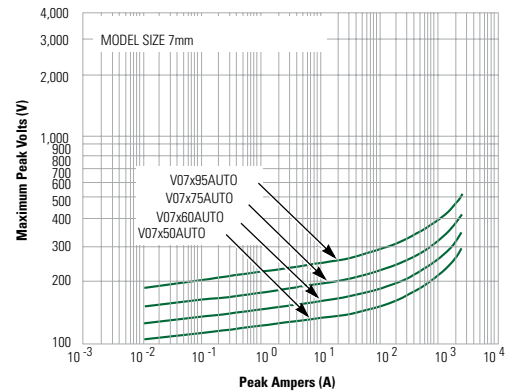
Maximum Clamping Voltage for 7mm Parts V07x50AUTO - V07x95AUTO
