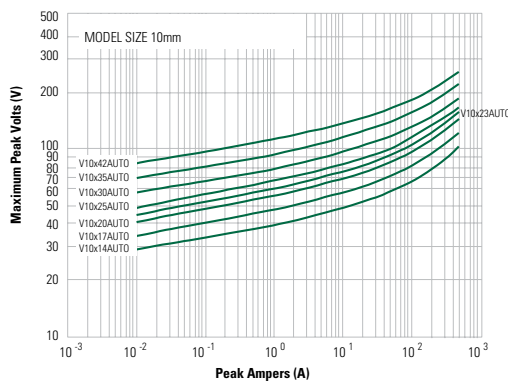
Maximum Clamping Voltage for 10mm Parts V10x14AUTO - V10x42AUTO
