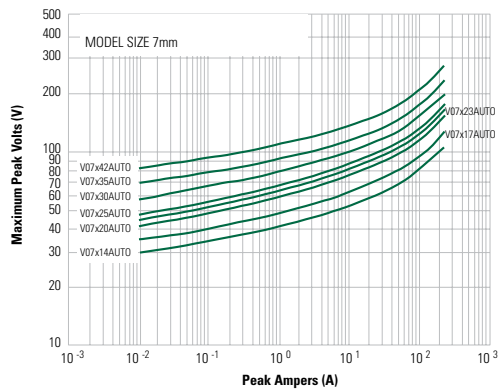
Maximum Clamping Voltage for 7mm Parts V07x14AUTO - V07x42AUTO
