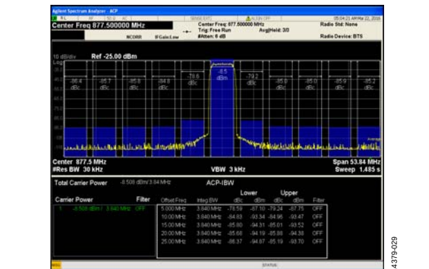
Figure 84. Single-Carrier W-CDMA at 877.5 MHz
