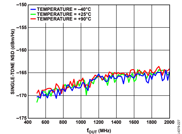
Figure 83. Single-Tone NSD Measured at 10% Offset from f_{OUT} vs. f_{OUT} over Temperature
