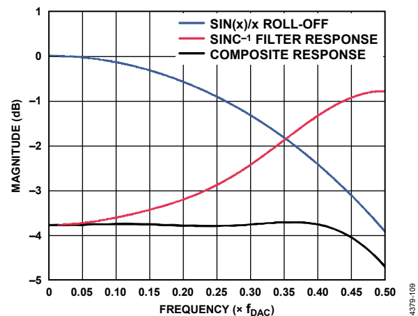
Figure 173. Responses of \sin(x)/x Roll-Off, the \text{Sinc}^{-1} Filter, and the Composite of the Two
