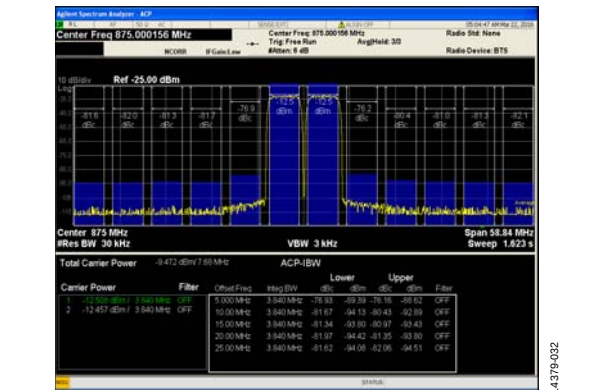
Figure 87. Two-Carrier W-CDMA at 875 MHz
