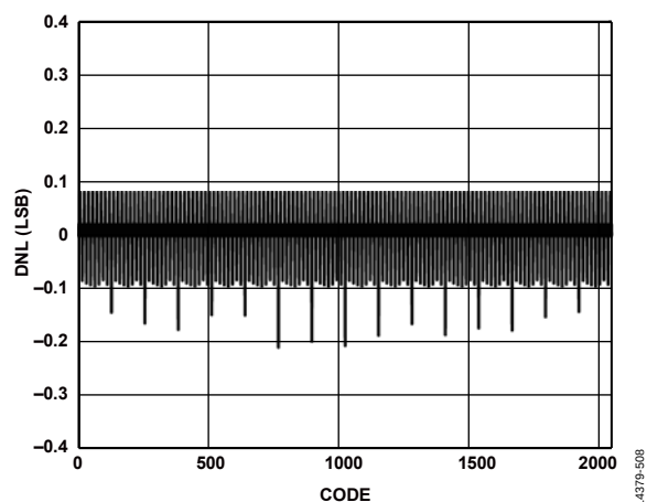
Figure 9. DNL, I_{OUTFS} = 20\text{ mA}
