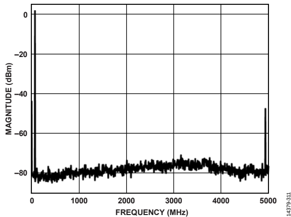
Figure 12. Single-Tone Spectrum at f_{OUT} = 70 MHz
