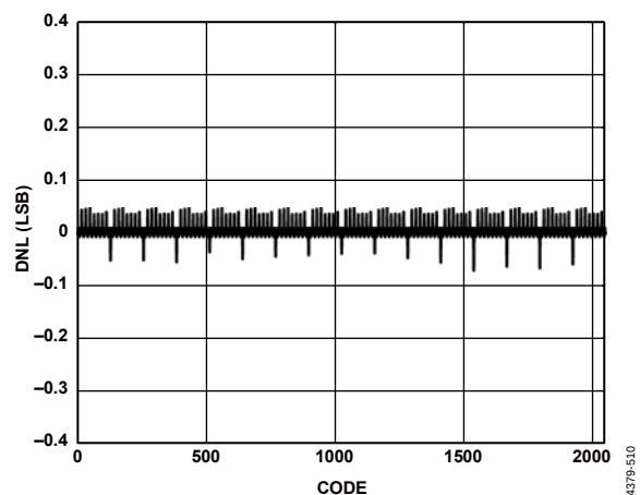
Figure 11. DNL, I_{OUTFS} = 40\text{ mA}
