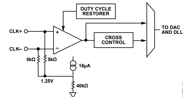
Figure 185. Clock Input
