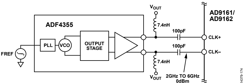
Figure 186. Possible Signal Chain for CLK± Input
