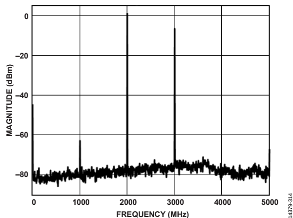
Figure 15. Single-Tone Spectrum at f_{OUT} = 2000 MHz
