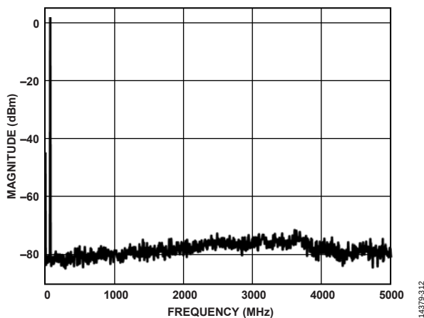
Figure 13. Single-Tone Spectrum at f_{OUT} = 70 MHz (FIR85 Enabled)
