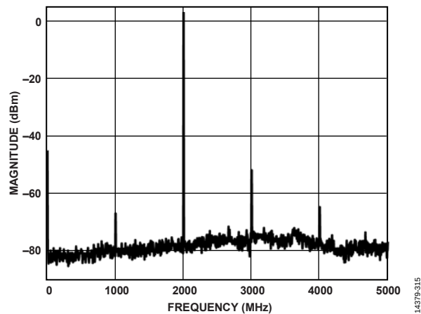
Figure 16. Single-Tone Spectrum at f_{OUT} = 2000 MHz (FIR85 Enabled)
