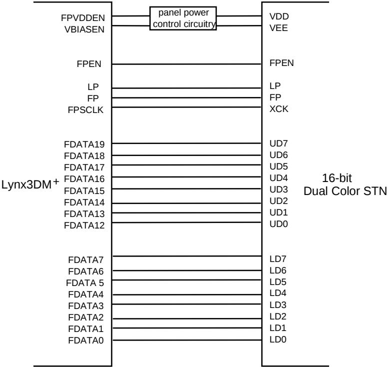
Figure 16: 16-bit DSTN Interface Configuration
