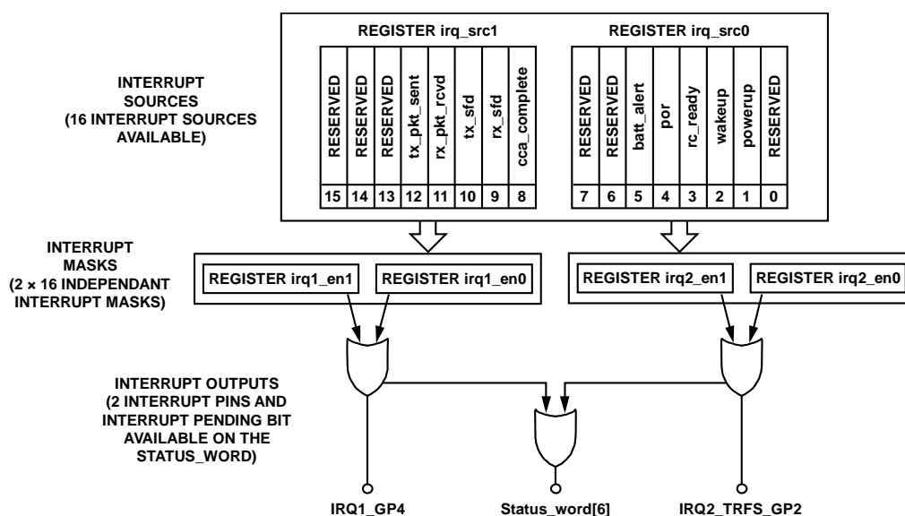
Figure 114. Interrupt Controller
