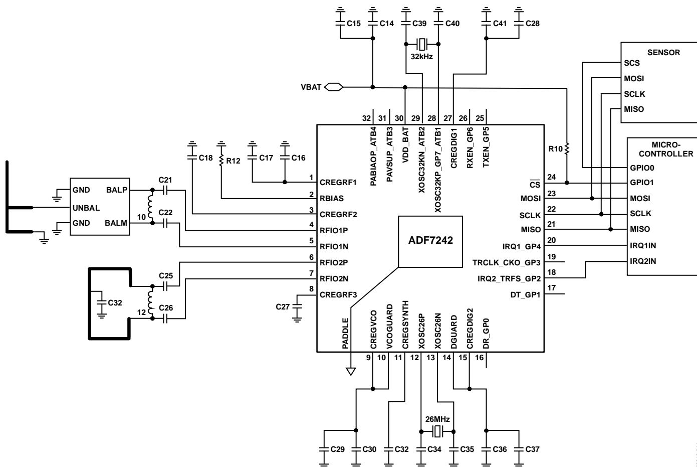
Figure 115. Typical ADF7242 Application Circuit Using Antenna Diversity
