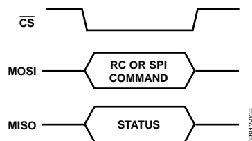
Figure 102. Command Write
