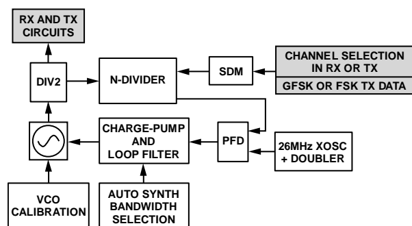
Figure 71. Synthesizer Architecture
