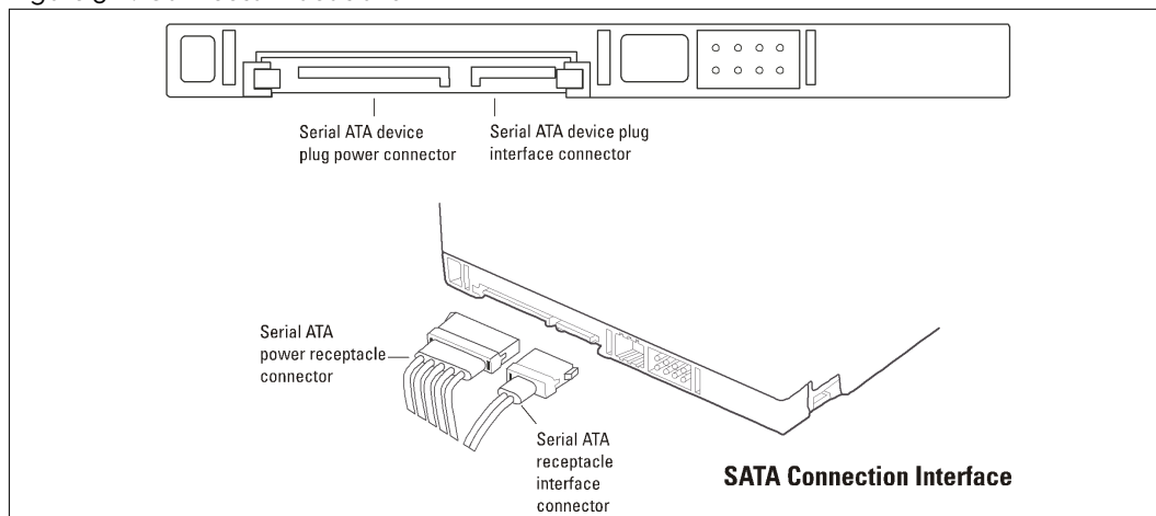
Figure 5-2. Connector Locations
