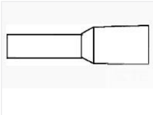
TE Part #1-966067-8 FER,WIRE,PL SLV,2.50/14,L18,BLUE,LP
