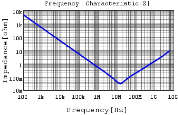
GCM155C71A474ME36 |Z| DCOV, 25degC
