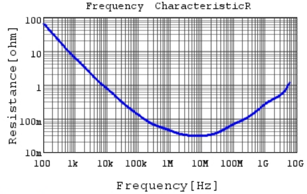
GCM155C71A474ME36 R DCOV, 25degC
