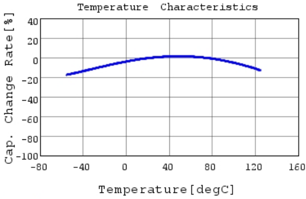
GCM155C71A474ME36 C-Temp. capchange, DC0.0V,
