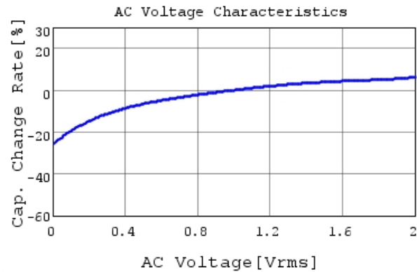
GCM155C71A474ME36 C-AC Voltage capchange, DC
