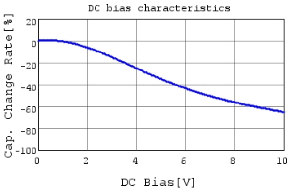
GCM155C71A474ME36 C-DC bias capchange, 25.00
