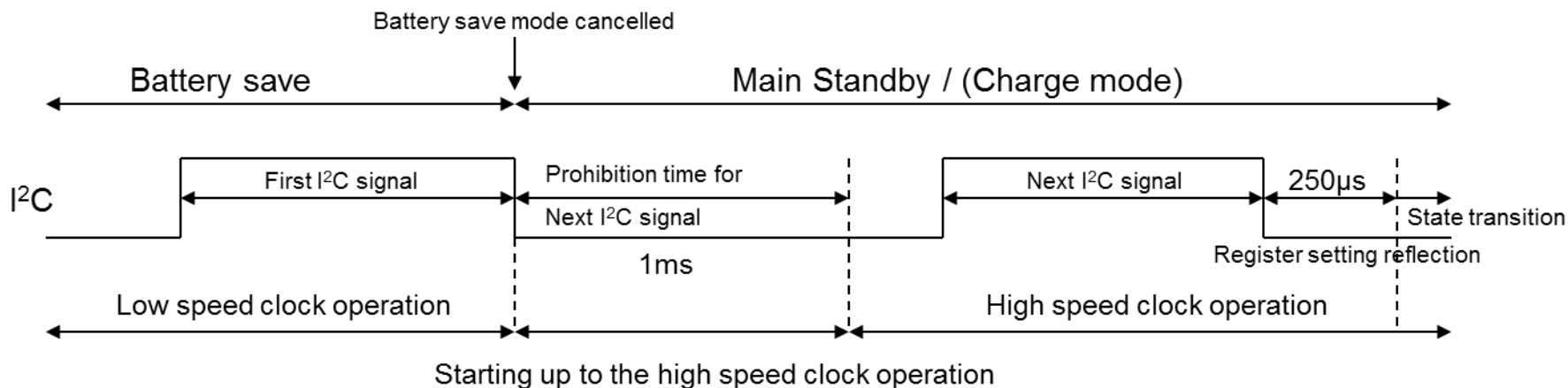
Figure 11-3 Timing chart: I 2 C
