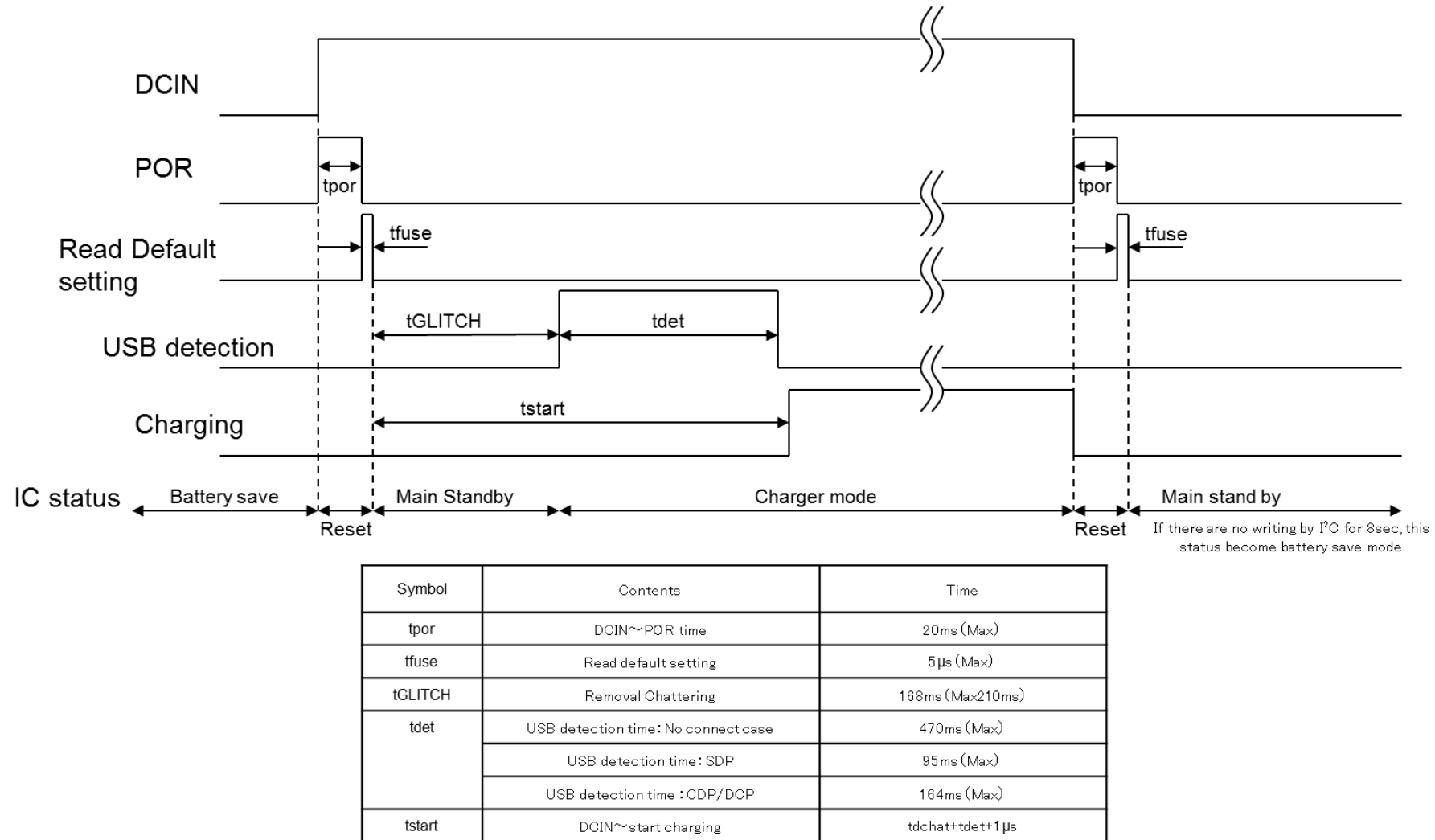
Figure 11-1 Timing chart: DCIN ON / OFF
