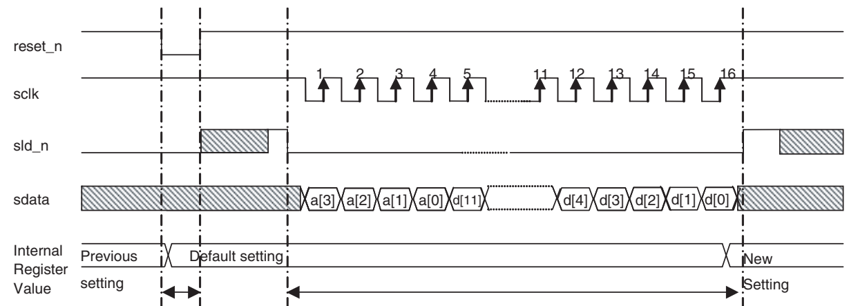
Figure 5-29. 3WSI Timing Diagram
