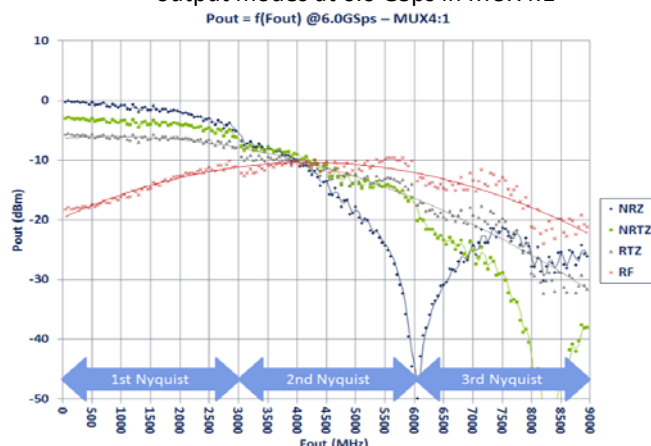
Figure 7-4. Pout vs Fout from 50 MHz to 8950 MHz in the 4 output modes at 6.0 GSps in MUX4:1
