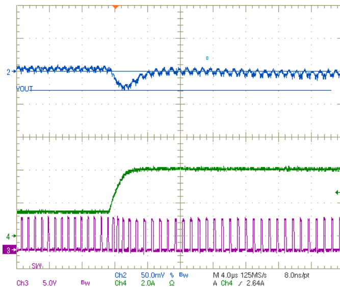
Figure 6. Step Load Rising Edge
