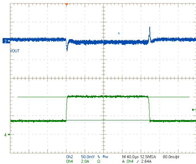
Figure 5. Step Load
