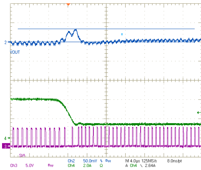
Figure 7. Step Load Falling Edge
