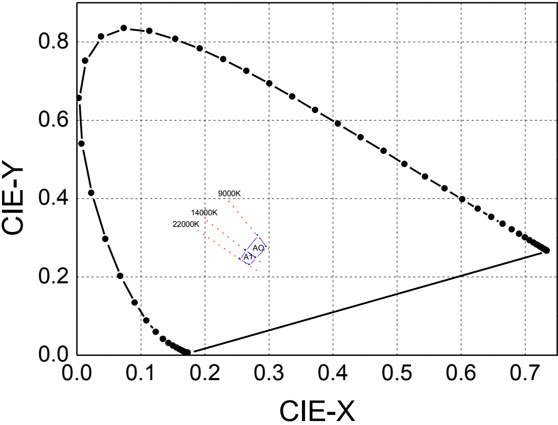
CIE Chromaticity Diagram
