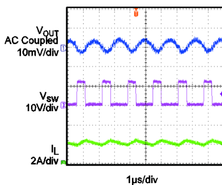
Output Voltage Ripple I_{OUT}=2A
