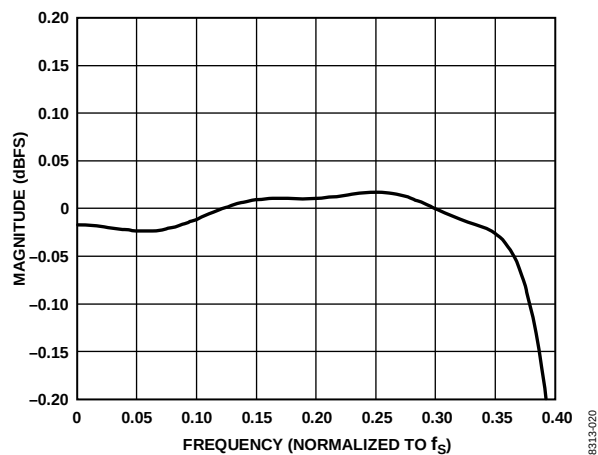
Figure 20. DAC Interpolation Filter Pass-Band Ripple, Double-Rate Mode, Normalized to f_s
