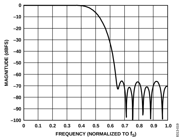
Figure 19. DAC Interpolation Filter, Double-Rate Mode, Normalized to f_s
