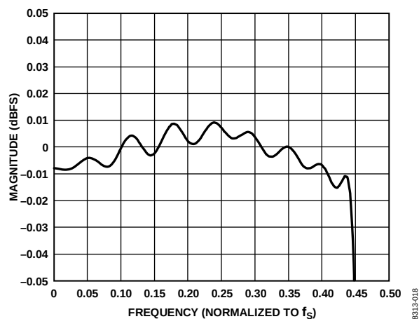
Figure 18. DAC Interpolation Filter Pass-Band Ripple, 128x Oversampling, Normalized to f_s
