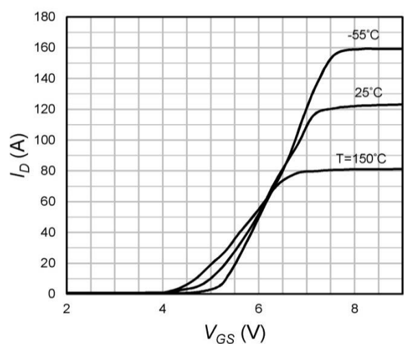
Fig.5 Transfer Characteristics
