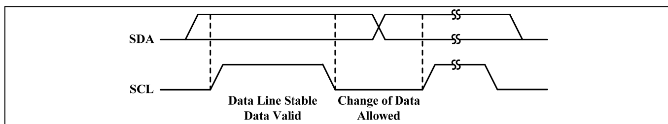
Figure 3 Bit transfer
