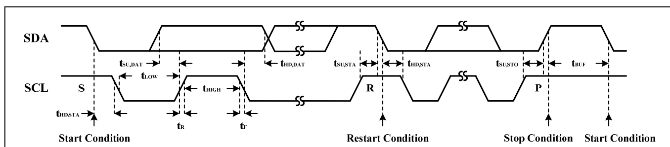
Figure 2 Interface timing
