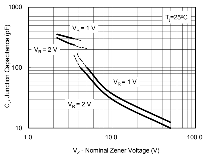
Fig. 4 Junction Capacitance VS. Nominal Zener Voltage
