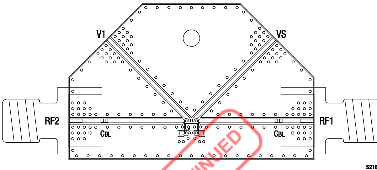
Figure 10. SKY13347-360LF Evaluation Board Assembly Diagram
