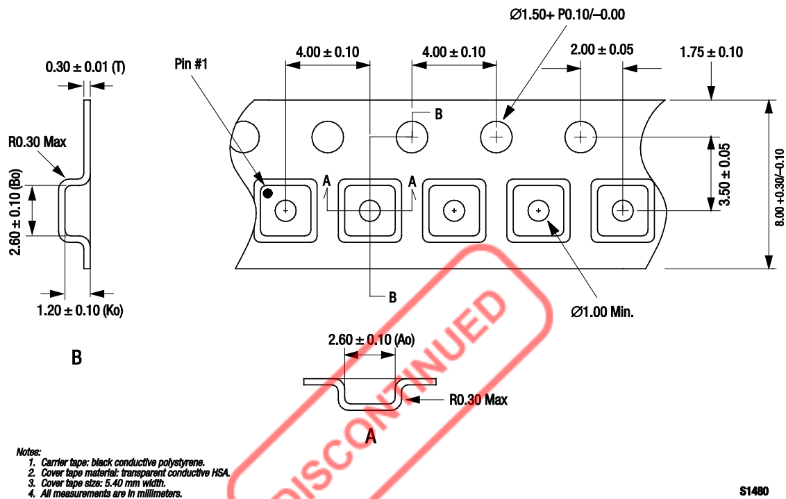
Figure 14. SKY13347-360LF Tape and Reel Dimensions
