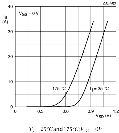
Fig 7. Source current as a function of source-drain voltage; typical values
