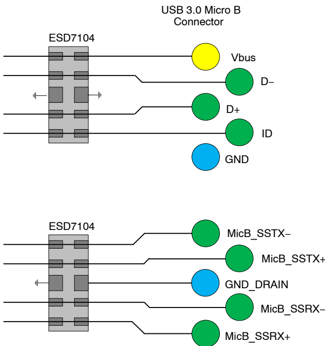
Figure 15. USB3.0 Micro B Connector Layout Diagram
