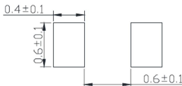
Figure 1. IN-S42AT Solder Pattern
