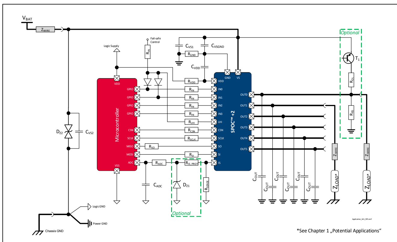
Figure 46 Application Diagram
