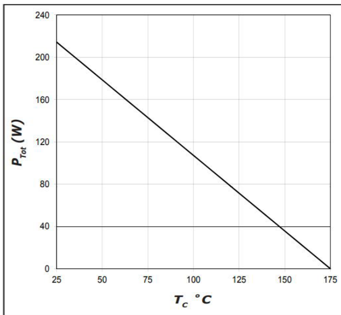
Figure 4 Power Derating
