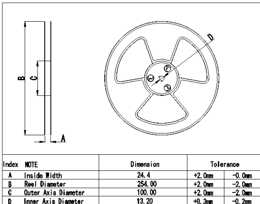
Figure 12. Reel Dimensions
