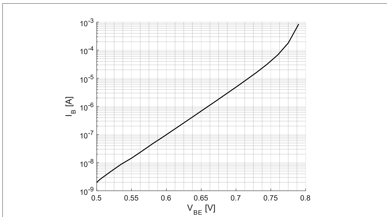
Figure 6 Base current I_B = f(V_{BE}) , V_{CE} = 8\text{ V}
