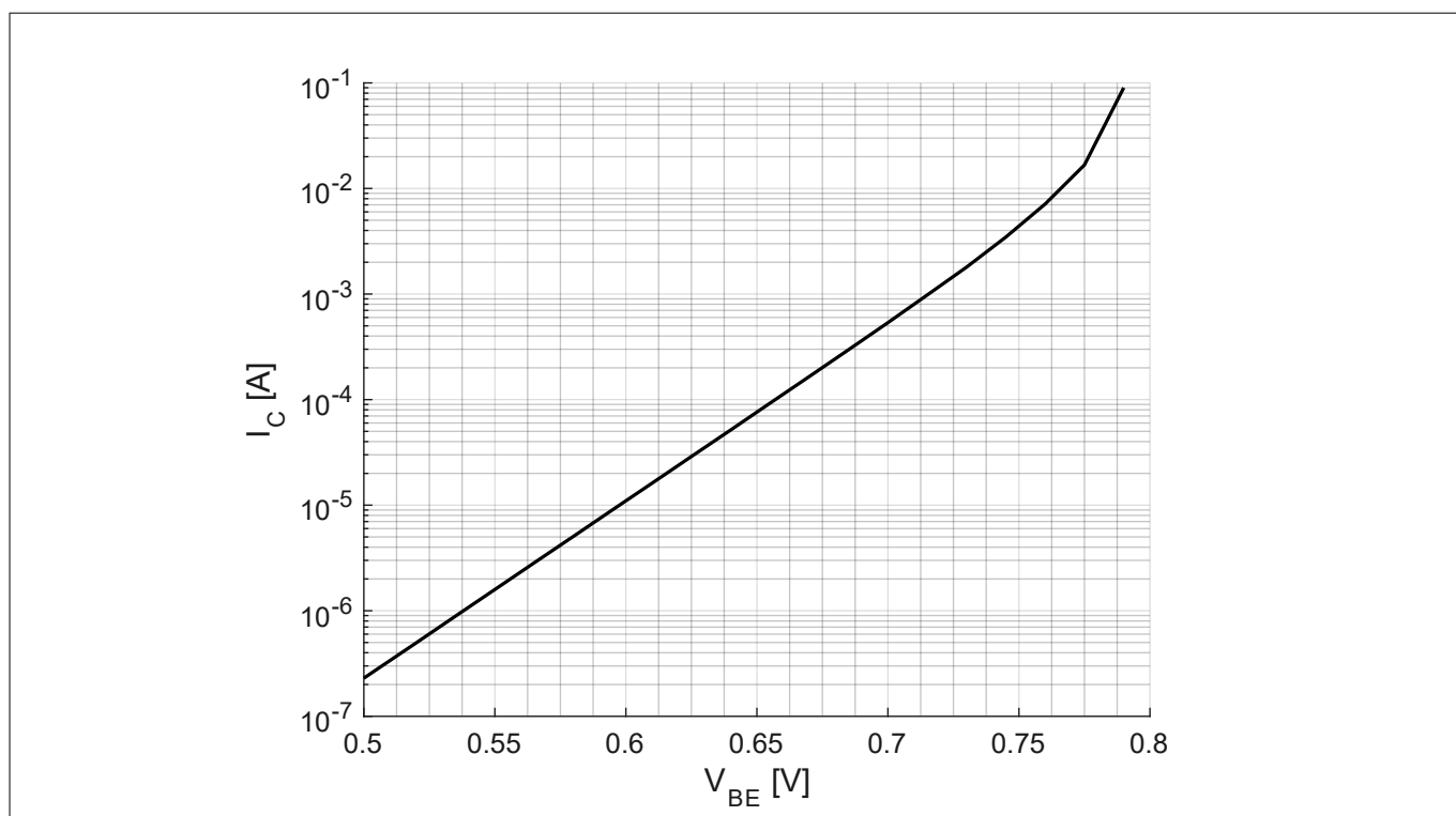
Figure 5 Collector current I_C = f(V_{BE}) , V_{CE} = 8\text{ V}
