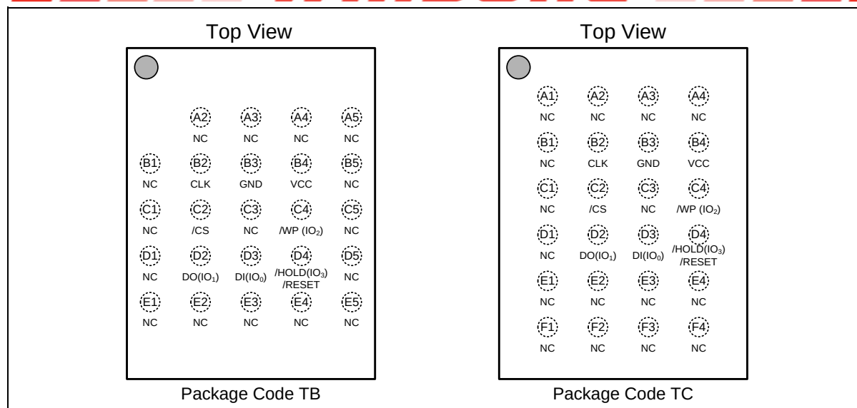
Figure 1d. W25Q32FV Ball Assignments, 24-ball TFBGA 8x6-mm (Package Code TB &amp; TC)
