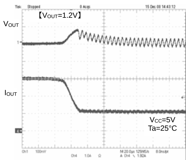
Figure 18. Transient Response ( I_o = 3A to 1A, 10\mu s )
