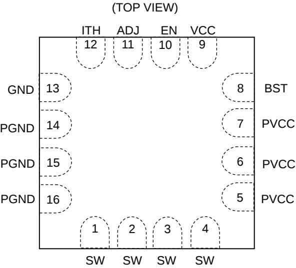
Figure 2. Pin Configuration
