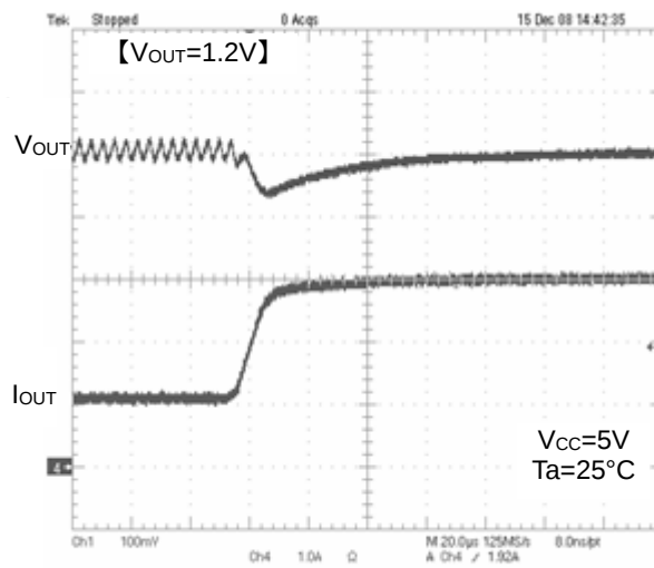
Figure 17. Transient Response ( I_o = 1A to 3A, 10\mu s )
