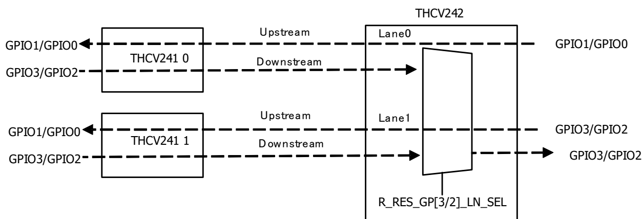
Figure 12. Through GPIO via Sub-Link transaction assignment with THCV241
