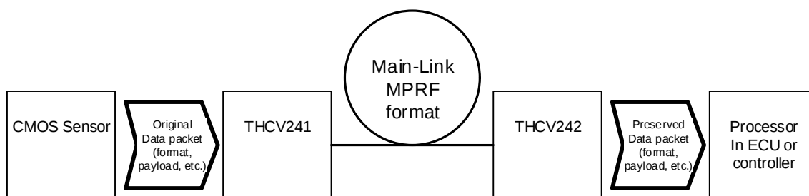
Figure 1. MPRF (Main-Link PRivate Format)
