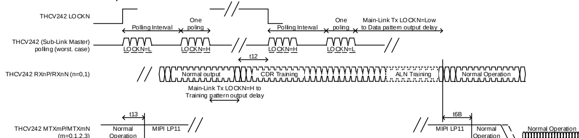
Figure 16. Re-Lock Sequence
