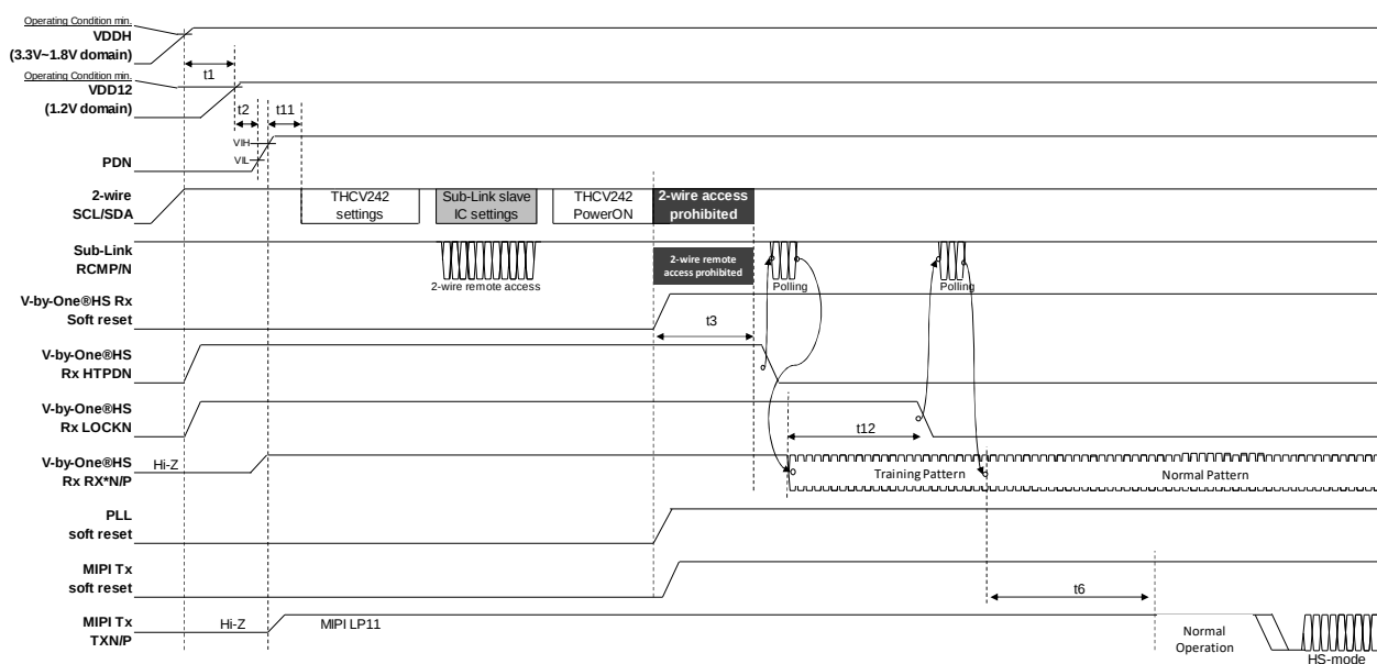
Figure 14. Power On Sequence procedure
