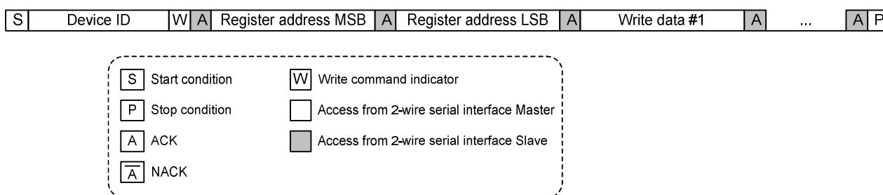
Figure 4. 2-wire serial I/F write to THCV242 local register protocol
