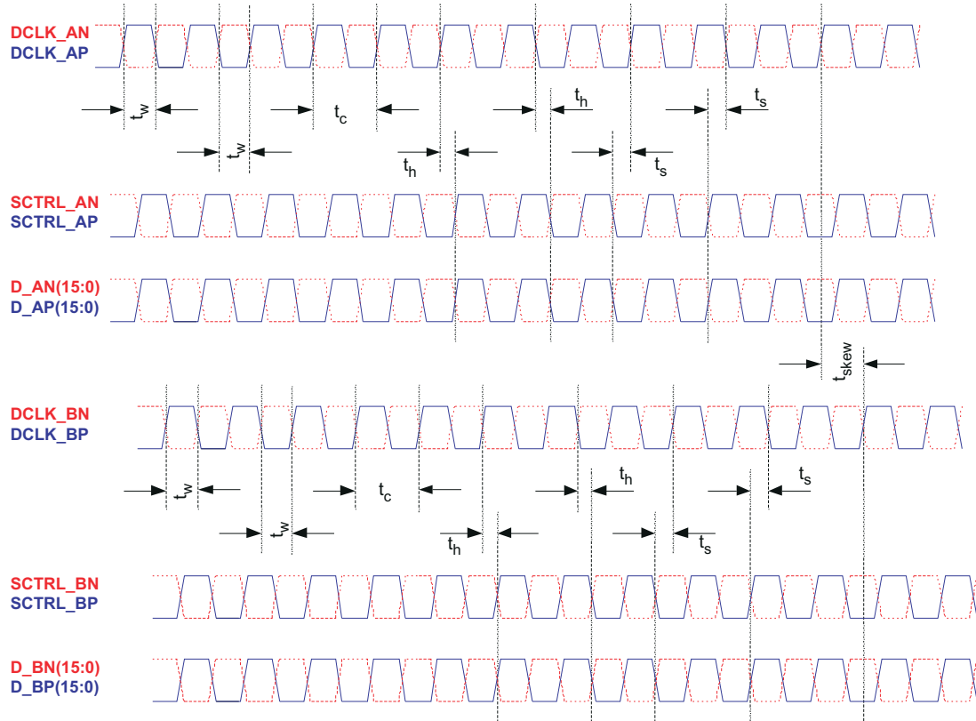
Figure 7-2. LVDS Timing Waveforms
