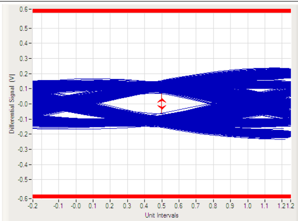
Figure 12. USB3.1 Gen 2 10-Gbps Eye Diagram (Bare Board)
