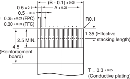
Applicable FPC/FFC Dimensions
