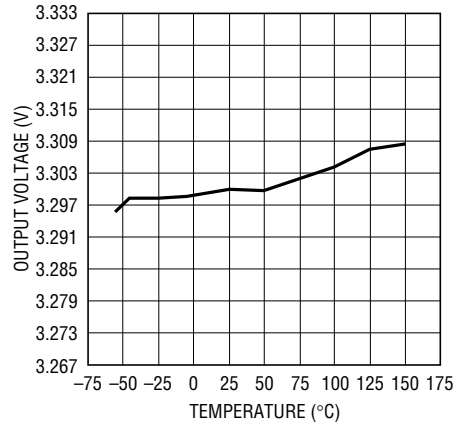
LT1575-3.3 V_{OUT} vs Temperature
