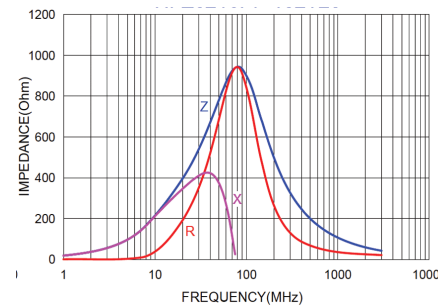
NCB-HD1206B102TR200F NCB-HD1206B102TR200QYF
