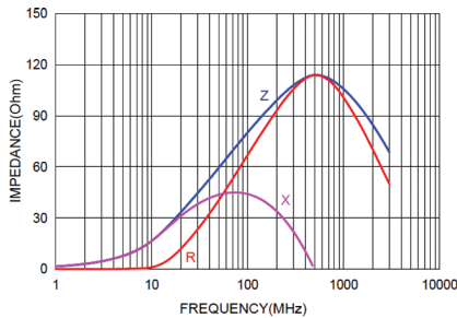
NCB-HD0402P800TR230F NCB-HD0402P800TR230QYF
