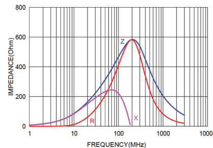
NCB-HD0402P471TR110F NCB-HD0402P471TR110QYF
