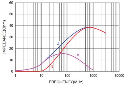
NCB-HD0805A300TR850F NCB-HD0805A300TR850QYF
