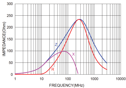
NCB-HD0805A181TR400F NCB-HD0805A181TR400QYF
