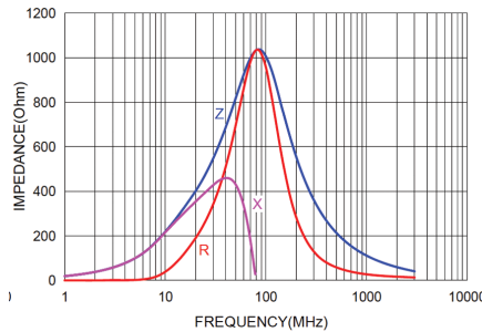
NCB-HD0805A102TR160F NCB-HD0805A102TR160QYF
