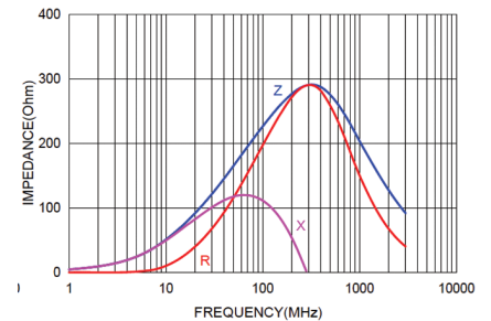
NCB-HD0402P221TR150F NCB-HD0402P221TR150QYF
