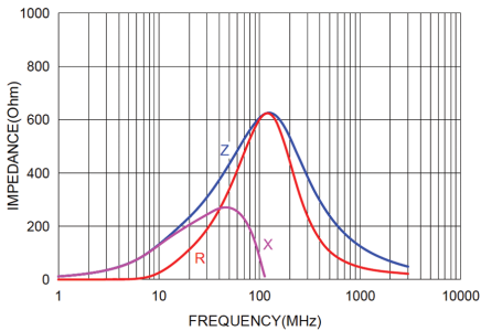
NCB-HD0805A601TR230F NCB-HD0805A601TR230QYF
