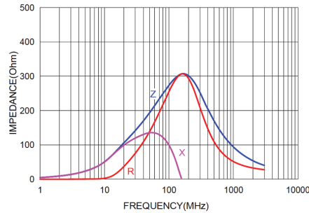
NCB-HD1206B271TR450F NCB-HD1206B271TR450QYF
