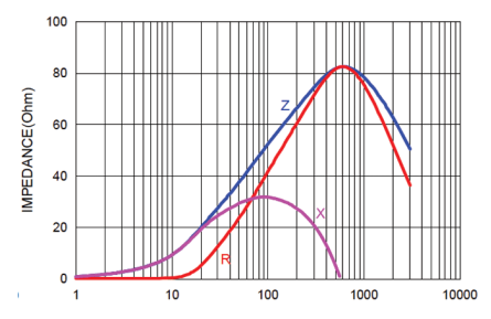
NCB-HD0402P600TR250F NCB-HD0402P600TR250QYF
