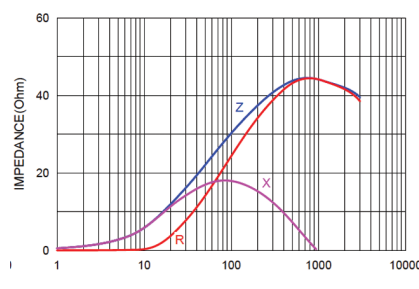
NCB-HD0402P300TR300F NCB-HD0402P300TR300QYF
