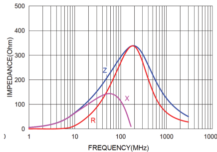
NCB-HD0805A331TR280F NCB-HD0805A331TR280QYF
