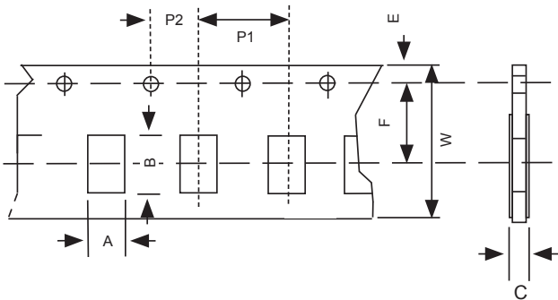
NCB-HD TAPE DIMENSIONS (mm)
