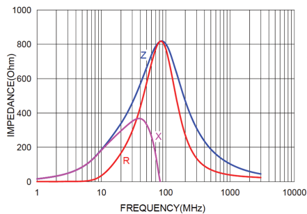
NCB-HD1206B801TR250F NCB-HD1206B801TR250QYF
