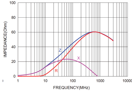
NCB-HD1206B500TR1200F NCB-HD1206B500TR1200QYF
