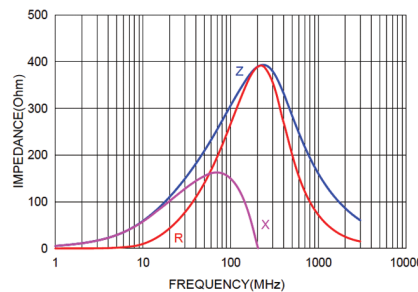
NCB-HD0402P301TR120F NCB-HD0402P301TR120QYF
