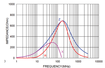
NCB-HD0402P601TR100F NCB-HD0402P601TR100QYF
