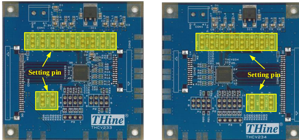
Figure 9 Position of Function Setting Pin
