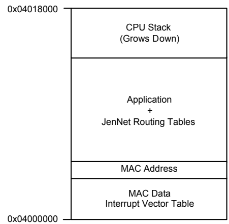
Figure 7: Typical RAM Contents
