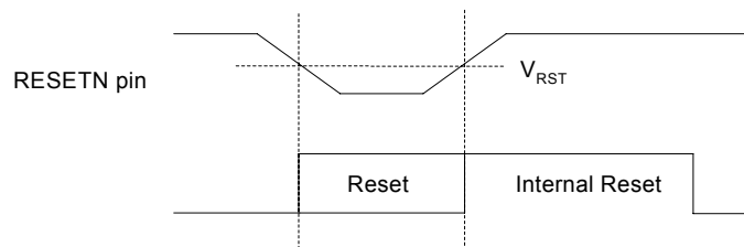
Figure 12: External Reset
