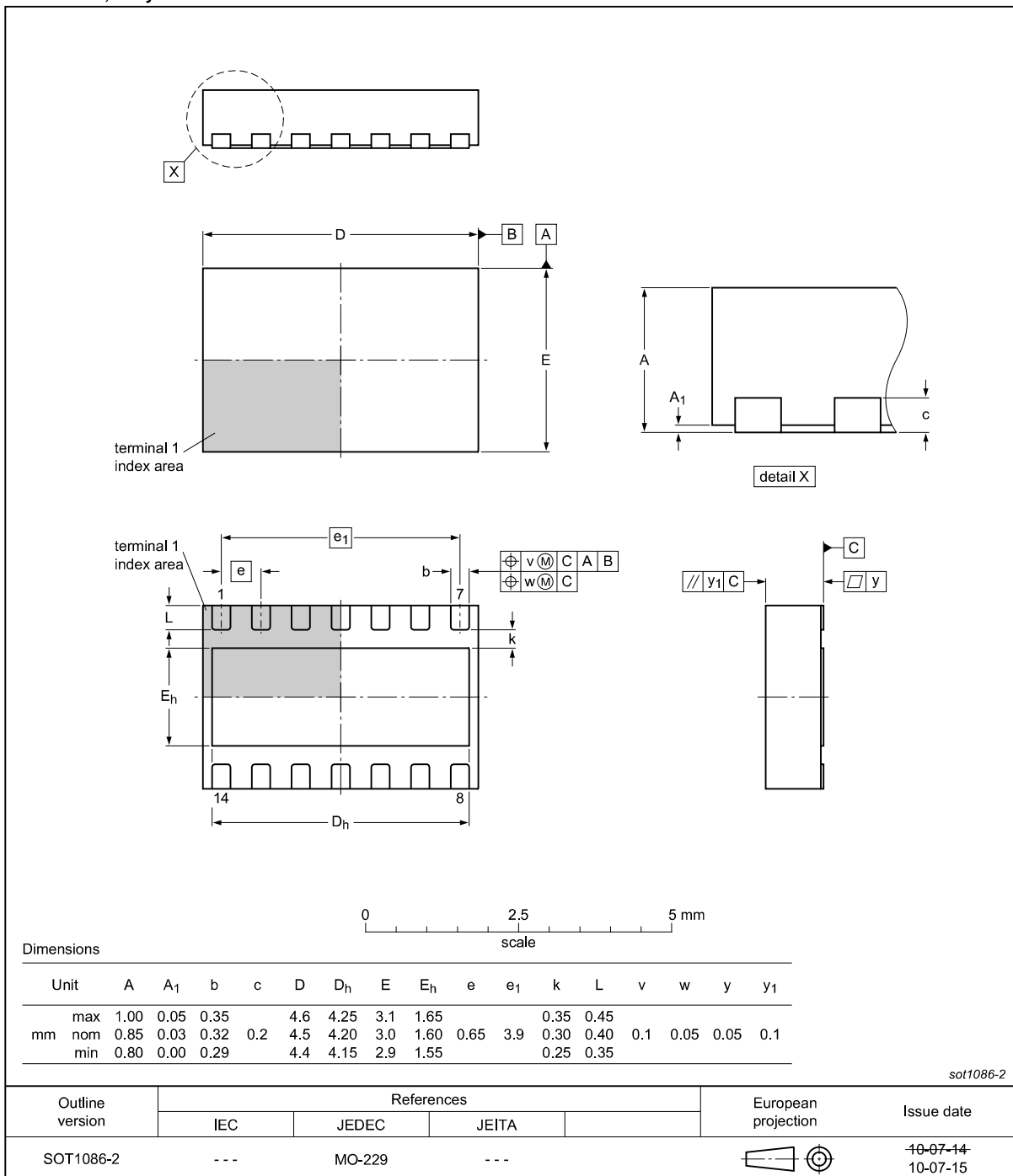
Figure 16. Package outline SOT1086-2 (HVSON14)
