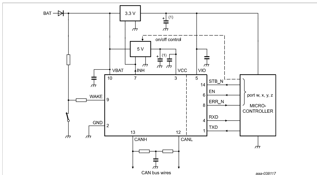
Figure 12. Typical TJA1463 application with a 3.3 V microcontroller
