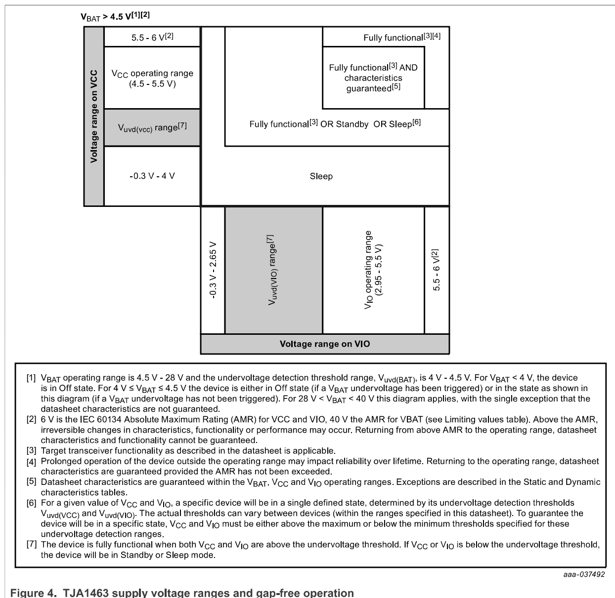
Figure 4. TJA1463 supply voltage ranges and gap-free operation
