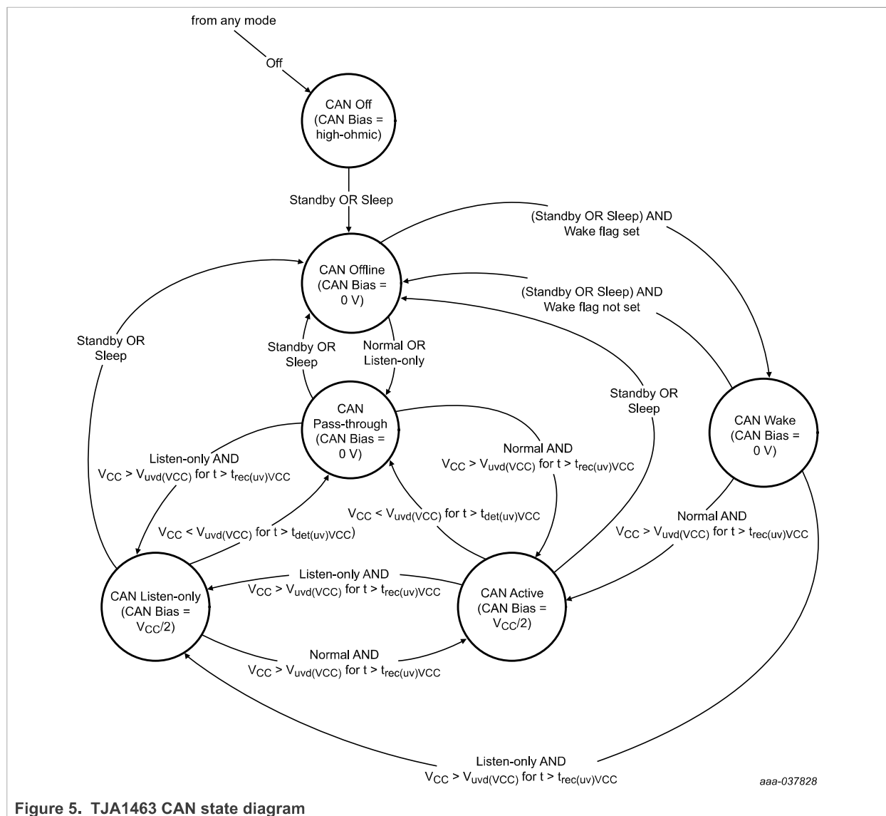
Figure 5. TJA1463 CAN state diagram
