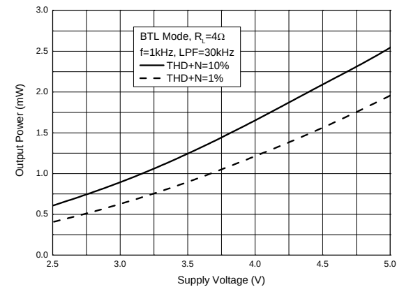
Output Power vs. Supply Voltage @ BTL Mode
