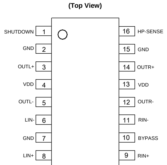
SOIC-16 (M Package)
