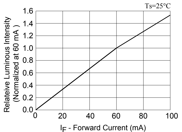
Fig.2 - Relative Luminous Intensity vs. Forward Current
