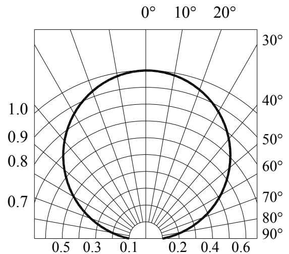
Fig.6 - Radiation Diagram
