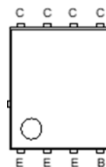
Top View Pin Configuration
