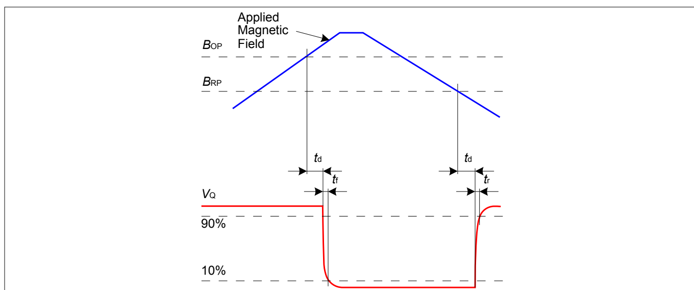
Figure 3 Timing diagram
