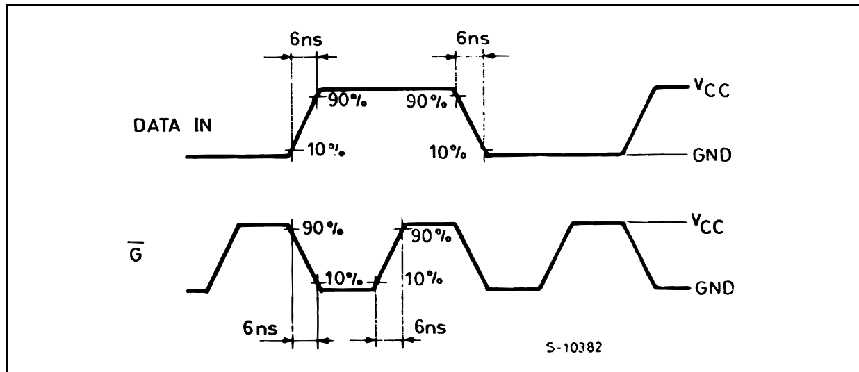
WAVEFORM 6 : INPUT WAVEFORMS ( f=1\text{MHz} ; 50% duty cycle)
