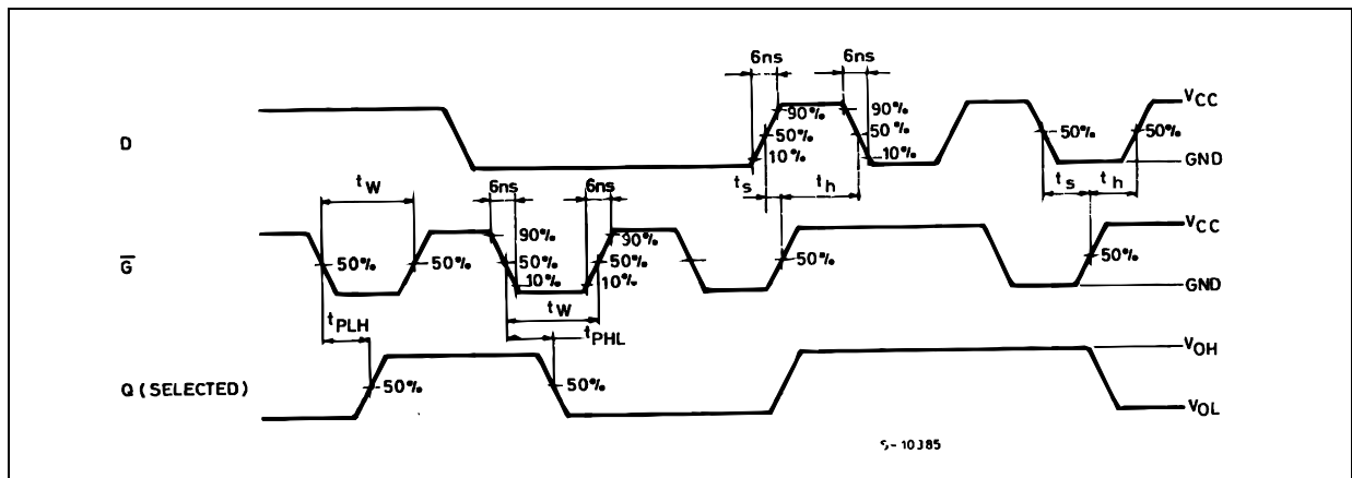
WAVEFORM 3 : MINIMUM PULSE WIDTH ( \overline{G} ), SETUP AND HOLD TIME (D TO \overline{G} ) ( f=1\text{MHz} ; 50% duty cycle)
