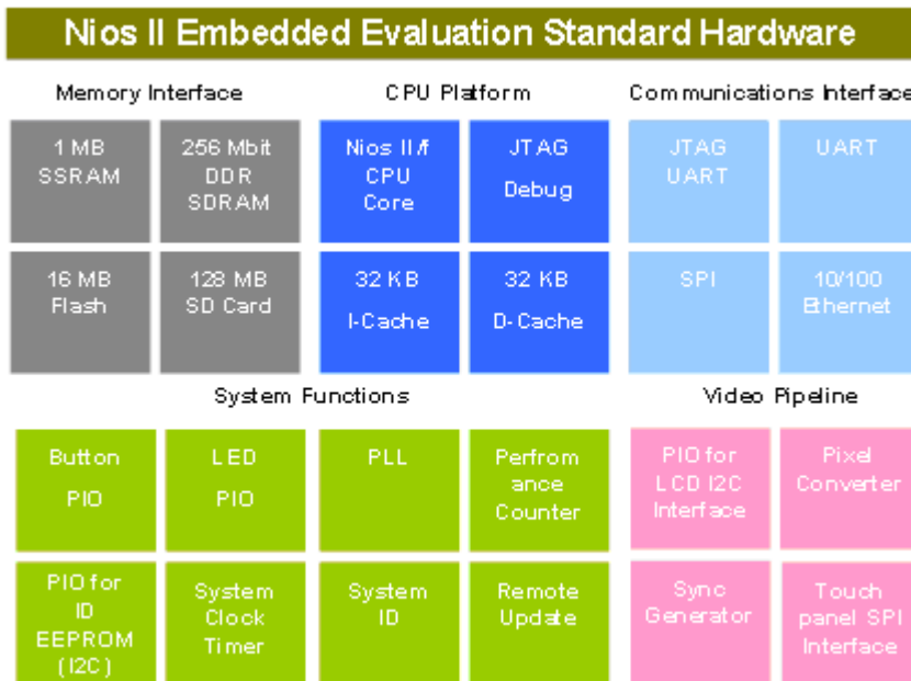
Figure 3–2. Nios II Embedded Evaluation Standard Hardware System Block Diagram
