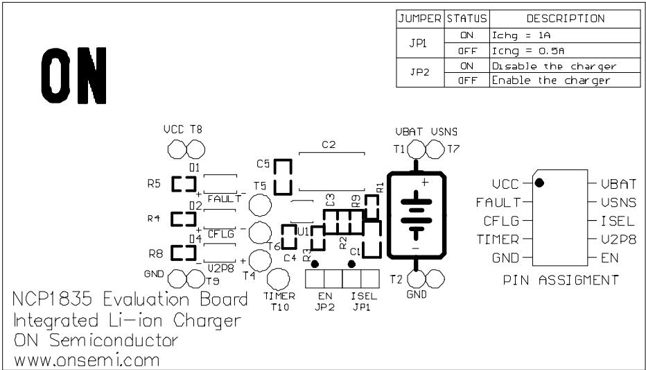
Figure 23. Silkscreen Layer
