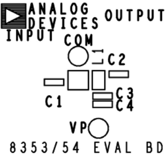
Figure 41. Silkscreen Top
