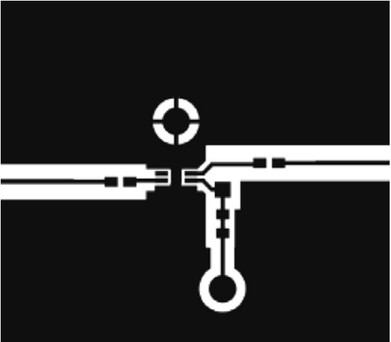
Figure 42. Component Side
