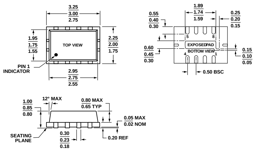
Figure 43. 8-Lead Lead Frame Chip Scale Package [LFCSP_VD] 2 mm × 3 mm Body, Very Thin, Dual Lead CP-8-1 Dimensions shown in millimeters
