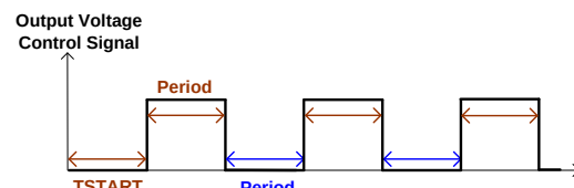
Figure 44. FCP-Single Communication Protocol Control Signal Waveform
