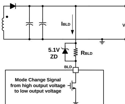
Figure 45. Output Bleeder Function
