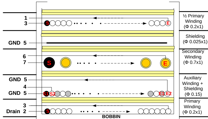
Figure 47. Transformer Diagram
