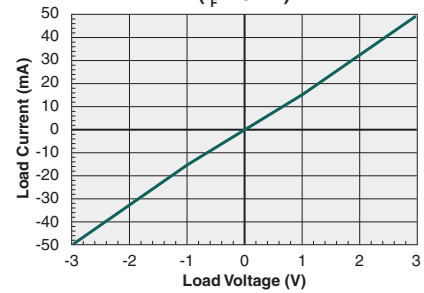
Typical Load Current vs. Load Voltage ( I_F=10\text{mA} )
