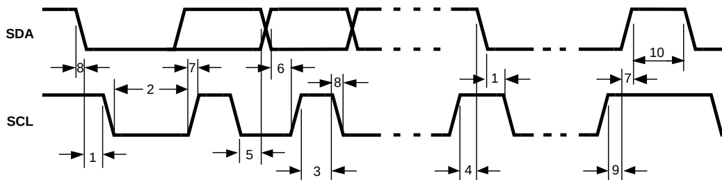
Figure 34. I²C Timing Diagram
