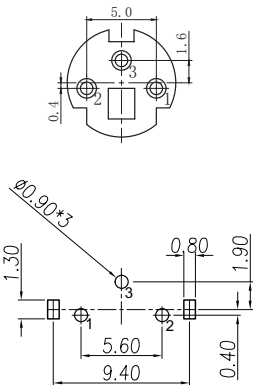
Recommended PCB Layout Bottom View (Date Codes prior to 03/03/2022)
