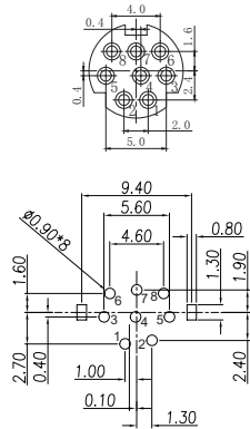
Recommended PCB Layout Bottom View (Date Codes prior to 03/03/2022)
