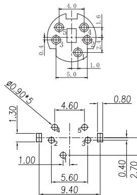
Recommended PCB Layout Bottom View (Date Codes prior to 03/03/2022)
